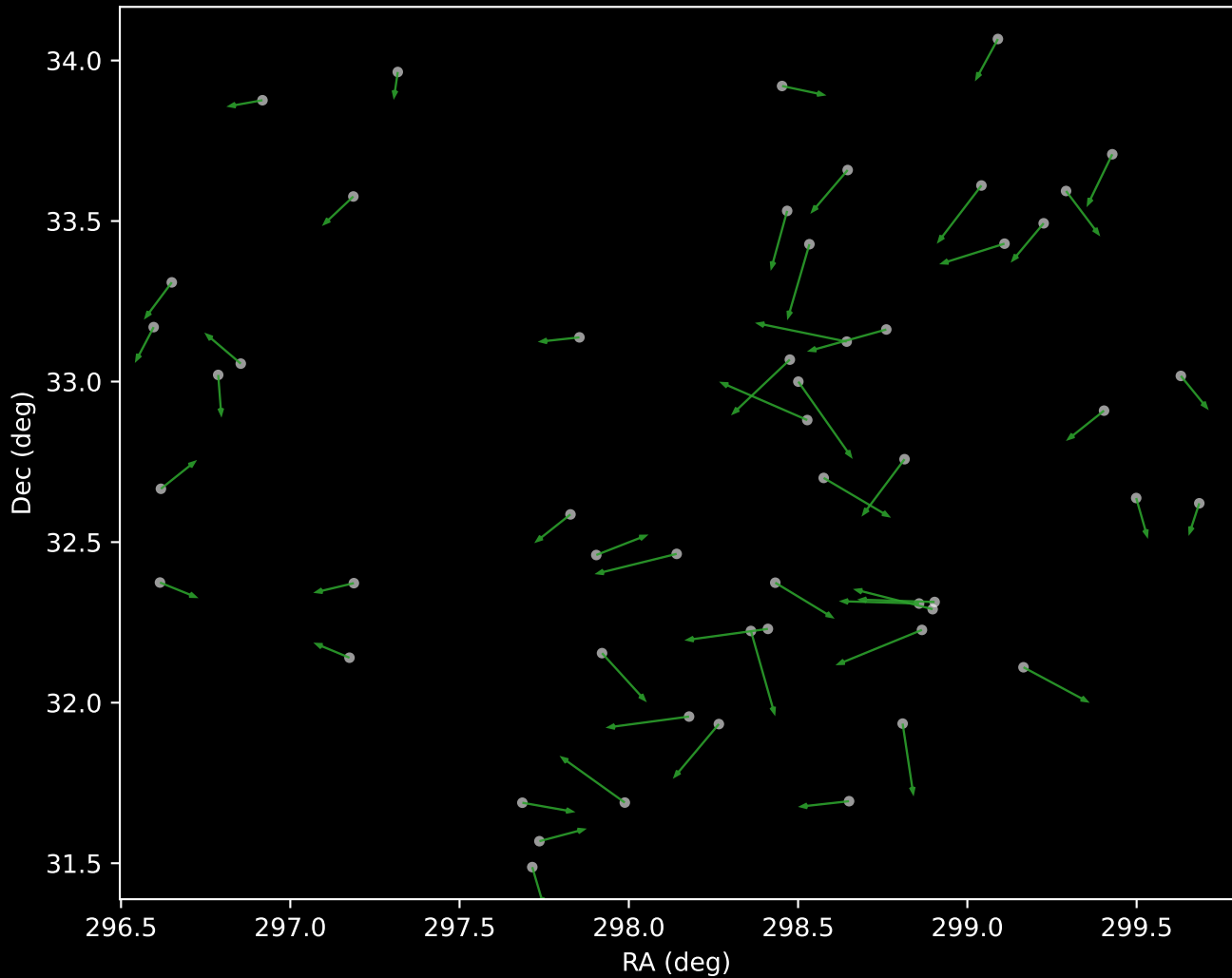
APOGEE DR17 Cluster 4 Proper Motion Vectors (n=53)
