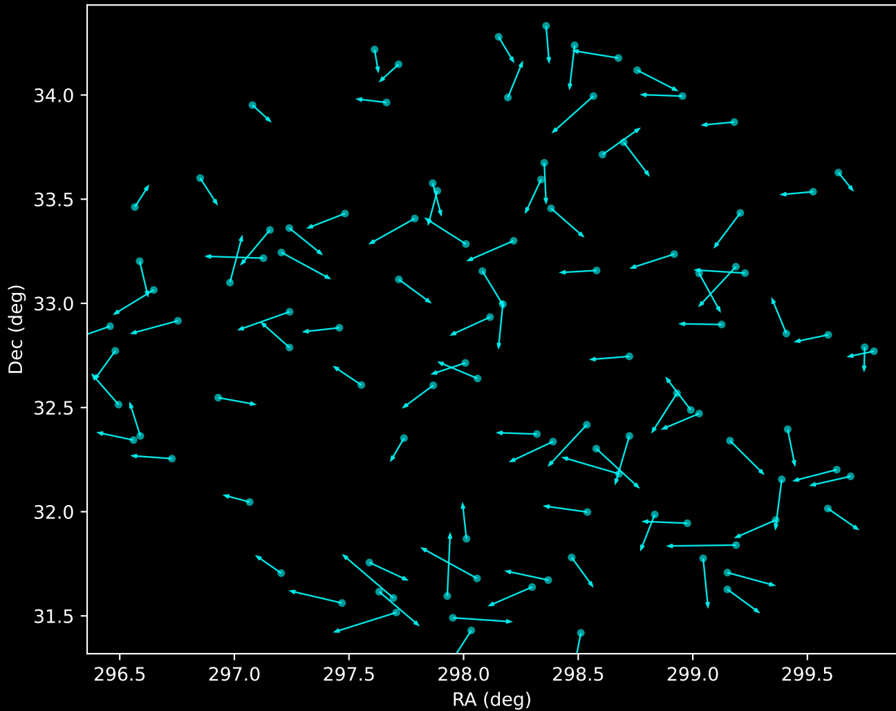
APOGEE DR17 Noise Stream Proper Motion Vectors (n=106)
