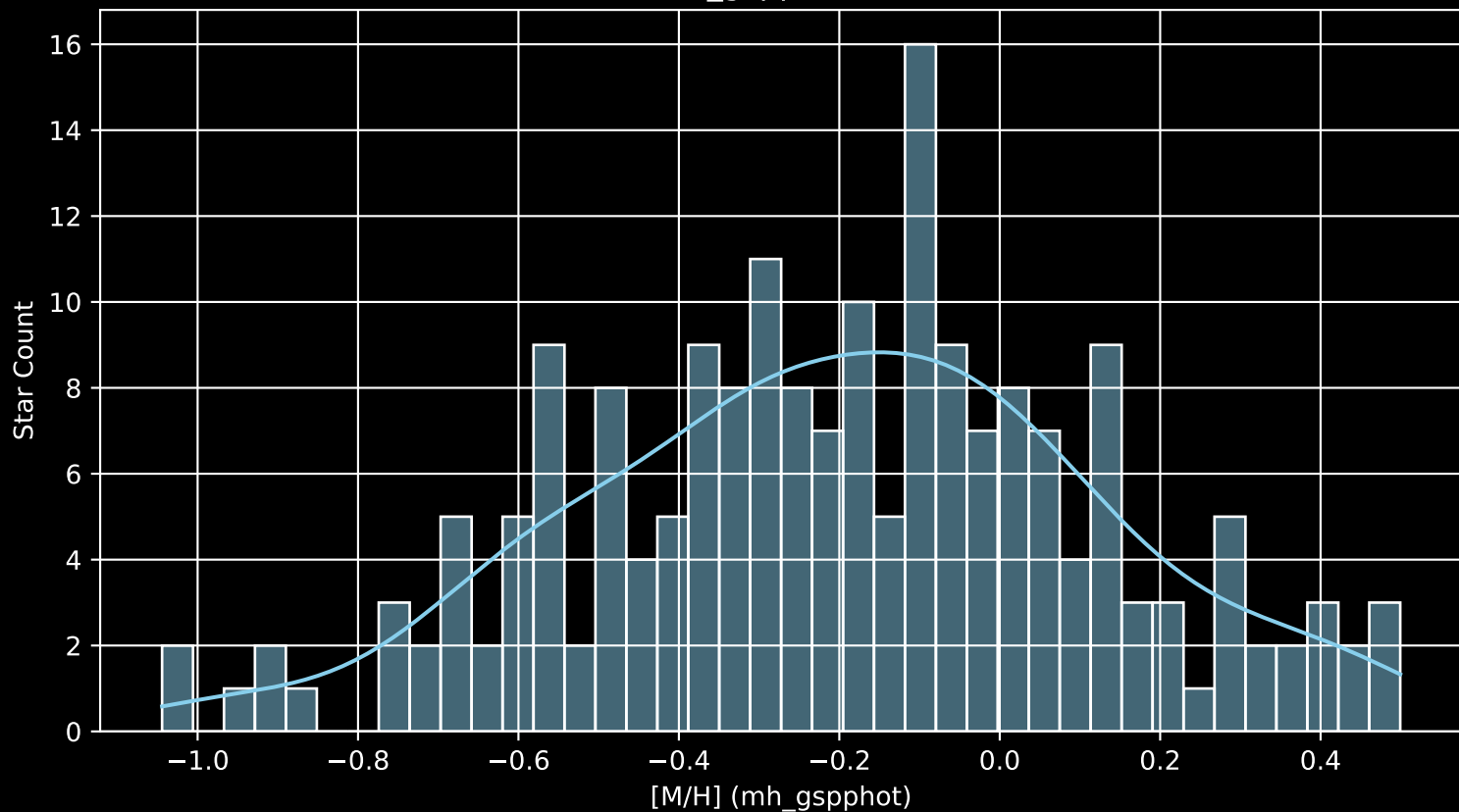
APOGEE DR17 Field: [085+83_MGA [M/H] (mh_gspphot) (n= 193)
