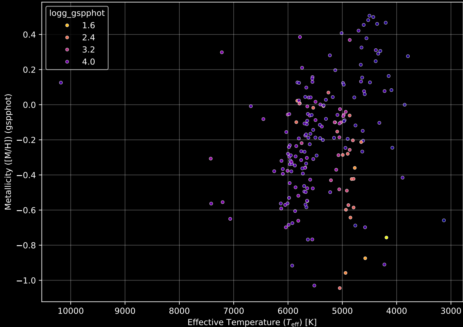
APOGEE DR17 Field: [085+83_MGA] Stellar Population Parameters (n= 194)
