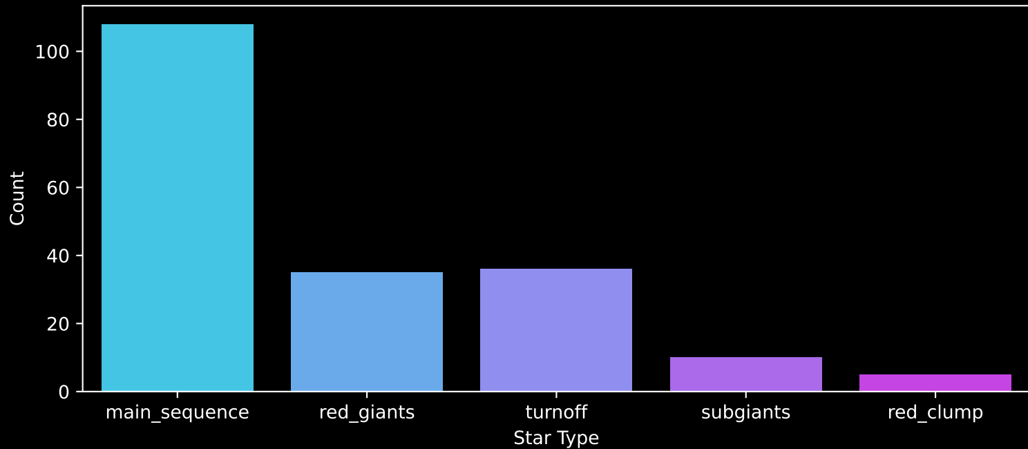
APOGEE DR17 Field: [085+83_MGA] Count plot of Star Type
