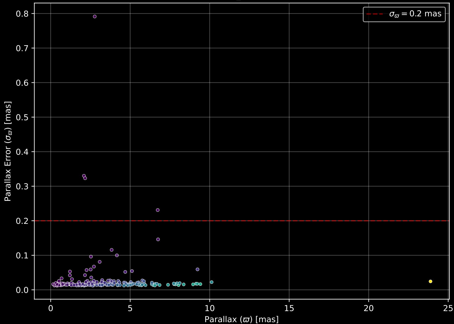
APOGEE DR17 Field: [085+83_MGA] Parallax Quality (n= 194)
