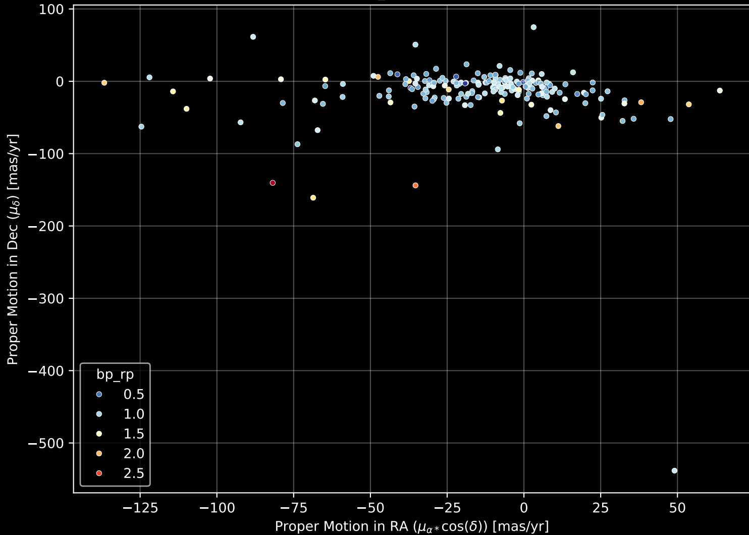
APOGEE DR17 Field: [085+83_MGA] Proper Motion Diagram (n= 194)
