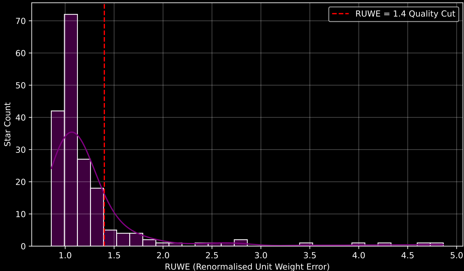
GAPOGEE DR17 Field [085+83_MGA] RUWE Distribution (n= 186)
